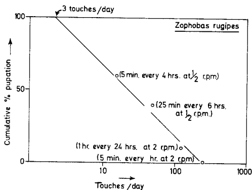
Fig. 5 Relation between the logarithm of the number of touches per day and the per cent of the larvae pupating within 20 days. Temporal distribution of stimulation is given in parentheses.
