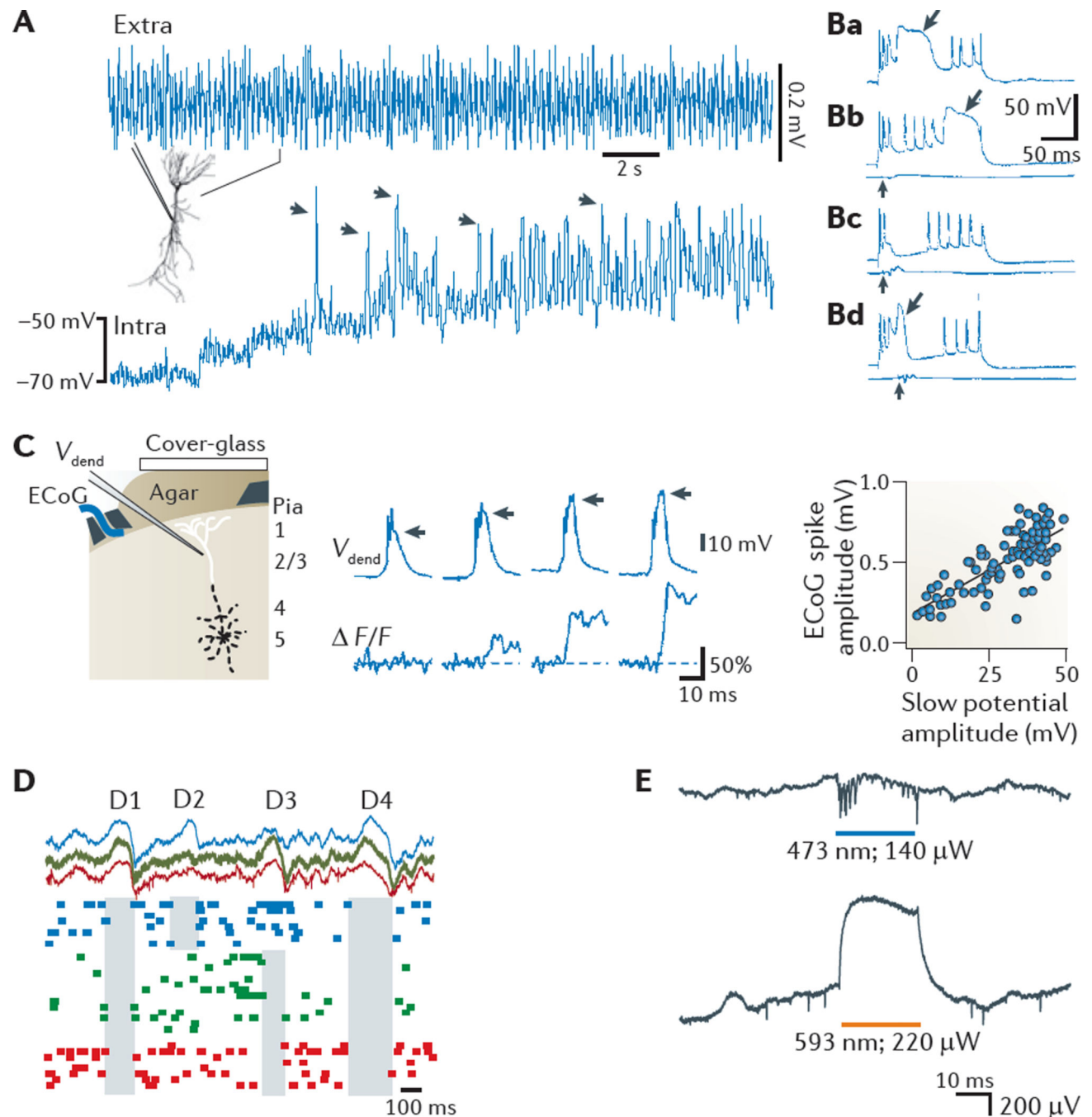
Figure 3. Non-synaptic contributions to the LFP
