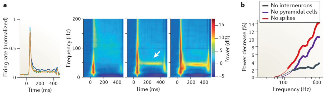
Figure 5. Spike contribution to the LFP
