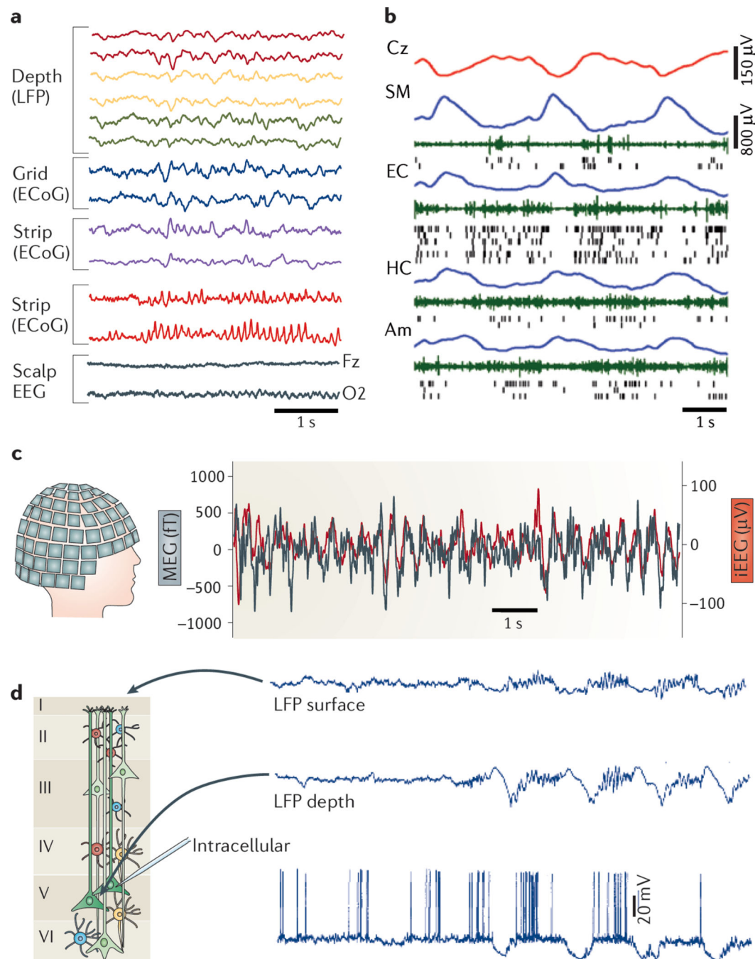
Figure 1. Extracellular traces using different recording methods are fundamentally similar
