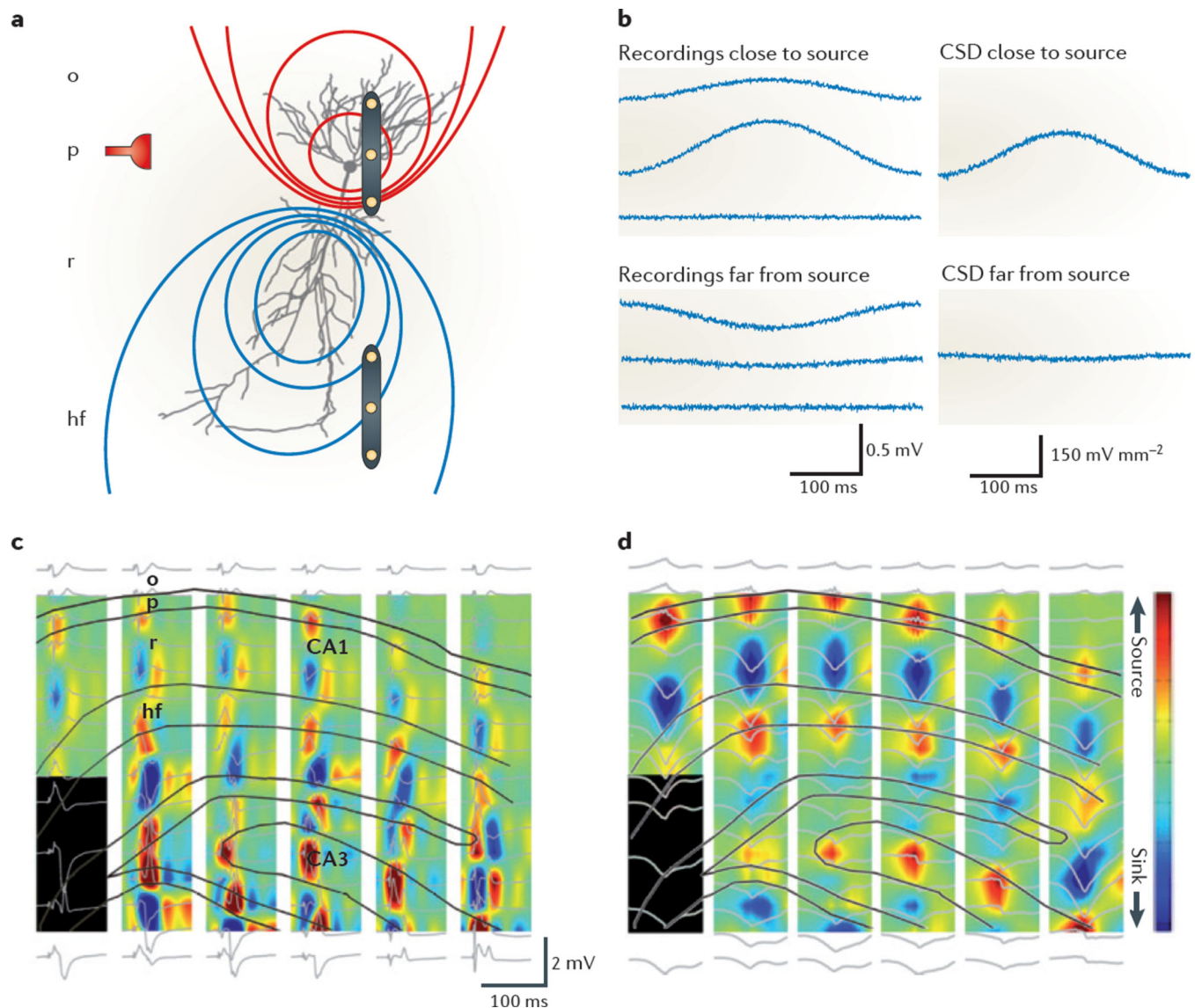
Figure 4. Identifying current sources
