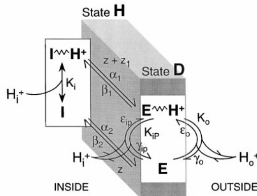
FIGURE 1. Titrateable voltage sensor models. (A) Gating currents were modeled as transitions between H and D connected by voltage-dependent rate constants \alpha and \beta . The charge carried by the titrateable voltage sensor in each transition between H and D is either z or z + z_1 , as determined by the equilibrium dissociation constant, pK ( K_i or K_o ), of the titrateable group and the surrounding pH ( H_i^+ or H_o^+ if the titrateable group gets exposed to the internal or external solution, respectively). Since the S4 segment, which contains most of the voltage sensing residues, is positively charged, depolarization of the membrane (gray box) moves the voltage sensor from the inside of the membrane towards the outside, thereby moving charge z or z + z_1 , in the transition. (B) The titrateable voltage sensor model shown in A was extended to incorporate the formation of a one-ion proton pore at depolarized potentials. In the D states, the titrateable residue has access to both the internal and external solutions simultaneously, and this creates a proton pathway through the membrane. Proton binding in the D states from the external solution depends on the dissociation constant, pK_o ( K_o = \gamma_o/\epsilon_o ) and the external pH ( H_o ); binding from the internal solution depends on pK_{ip} ( K_{ip} = \gamma_{ip}/\epsilon_{ip} ) and pH_i .
